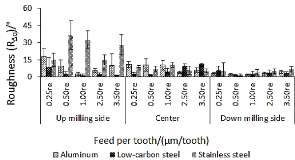
Figure 4. R_{\Delta q} parameter graph to 50 \mu\text{m} depth of cut.
