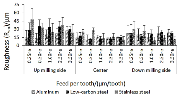
Figure 3. R_{sm} parameter graph to 50 \mu\text{m} depth of cut.
