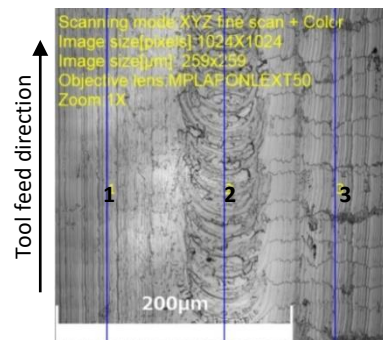
Figure 1. View from the top of the channel. Roughness measured in (1) up milling side, (2) center and (3) down milling side of microchannels surface.
