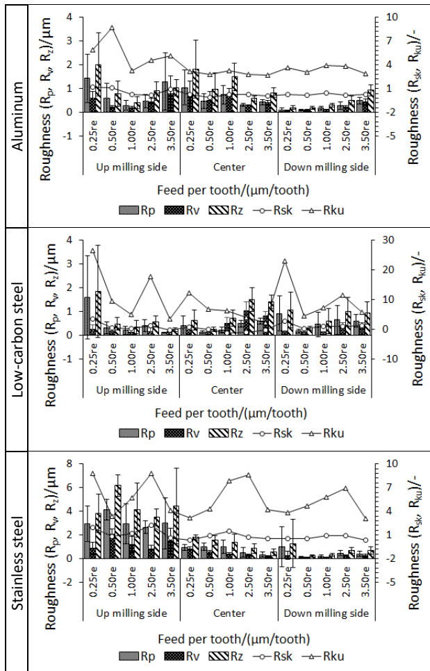
Figure 2. R_p , R_v , R_z , R_{sk} and R_{ku} parameters graphs to 50 \mu\text{m} depth of cut.
